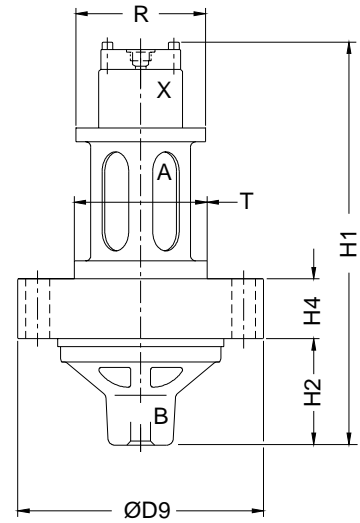
Model 'B' Tank Mounting
