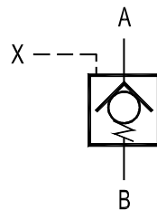
Hydraulic Symbol
